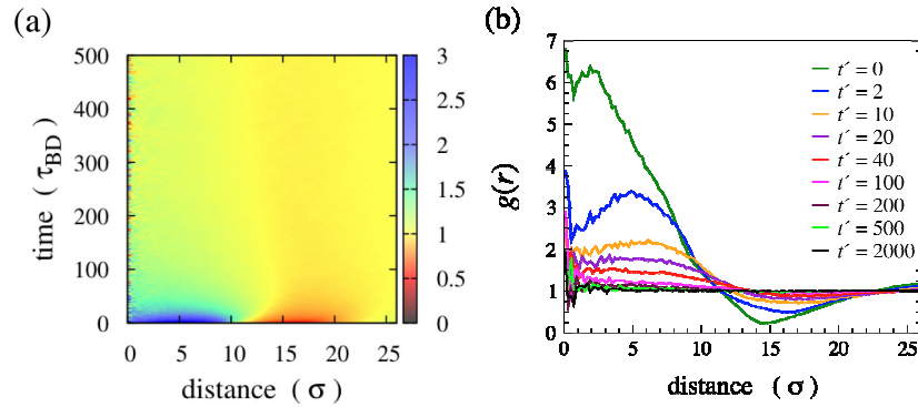
Figure 2. Radial chromosome density function, g(r) , averaged over eight chromosomes. The abscissa is a distance from the center of mass of each chromosome. (a) Time evolution of radial density function for t < 500 \tau_{BD} . The ordinate is the simulation time in the unit of \tau_{BD} . (b) Radial density function at specific simulation times, t' = t/\tau_{BD} .
