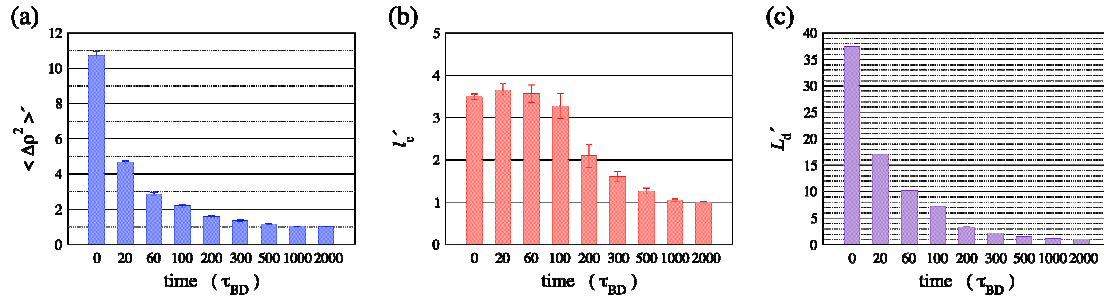
Figure 4. (a) Density variations \langle \Delta \rho^2 \rangle , (b) density correlation length l_c , and (c) disorder strength L_d for t=0-2000 \tau_{BD} . Each variable at a time ( t ) is normalized by its corresponding value at t=2000 \tau_{BD} . The data are calculated when the grid length of subcells is 120 nm in the x and y directions and 30 nm in the z direction.
