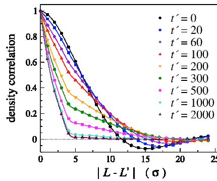
Figure 3. Normalized density correlation function, \langle \Delta\rho(L)\Delta\rho(L') \rangle / \langle \Delta\rho^2 \rangle , where \Delta\rho(z) = \langle \rho \rangle - \rho(z) and \langle \rho \rangle and \rho(z) are the average chromosome density and the density at z , respectively. The unit of length \sigma = 30 nm. In legends, t' = t/\tau_{BD} .
