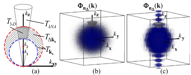
Fig. 3 Spatial-frequency space with k_z -axis antiparallel to \mathbf{k}_i . (a) Cross section of T_{\Delta\mathbf{k}_s} , T_{k\text{NA}} , and their interception, T_{3-D} ; (b) PSD of the RI fluctuation (blue) and T_{3-D} (gray) when the sample can be considered infinite (i.e., the LSs of internal organization are much smaller than sample thickness L ); and (c) when the sample is finite. Reproduced with permission from Ref. 19, courtesy of Phys. Rev. Lett.
