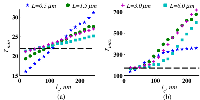
Fig. 8 Dependence of (a) r_{\min} and (b) r_{\max} corresponding to the 5% threshold on L and l_c . Black dashed lines indicate r_{\min} = 22 \text{ nm} and r_{\max} = 171 \text{ nm} corresponding to L = \infty . Reproduced with permission from Ref. 21, courtesy of Opt. Lett.
