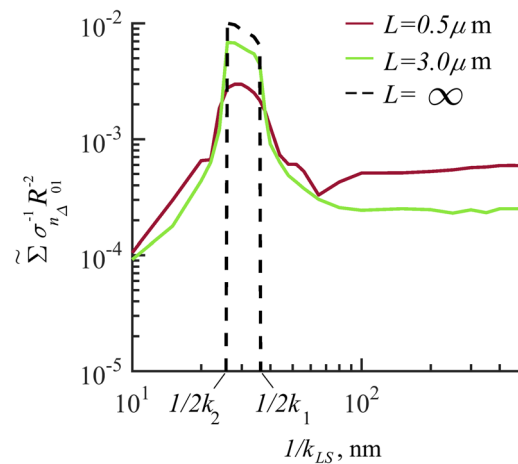
Fig. 6 \tilde{\Sigma} / \sigma_{n_A} R_{01}^2 as a function of the spatial frequency of RI fluctuations for samples with different thicknesses (all wavenumbers evaluated in vacuum). Reproduced with permission from Ref. 21, courtesy of Opt. Lett.
